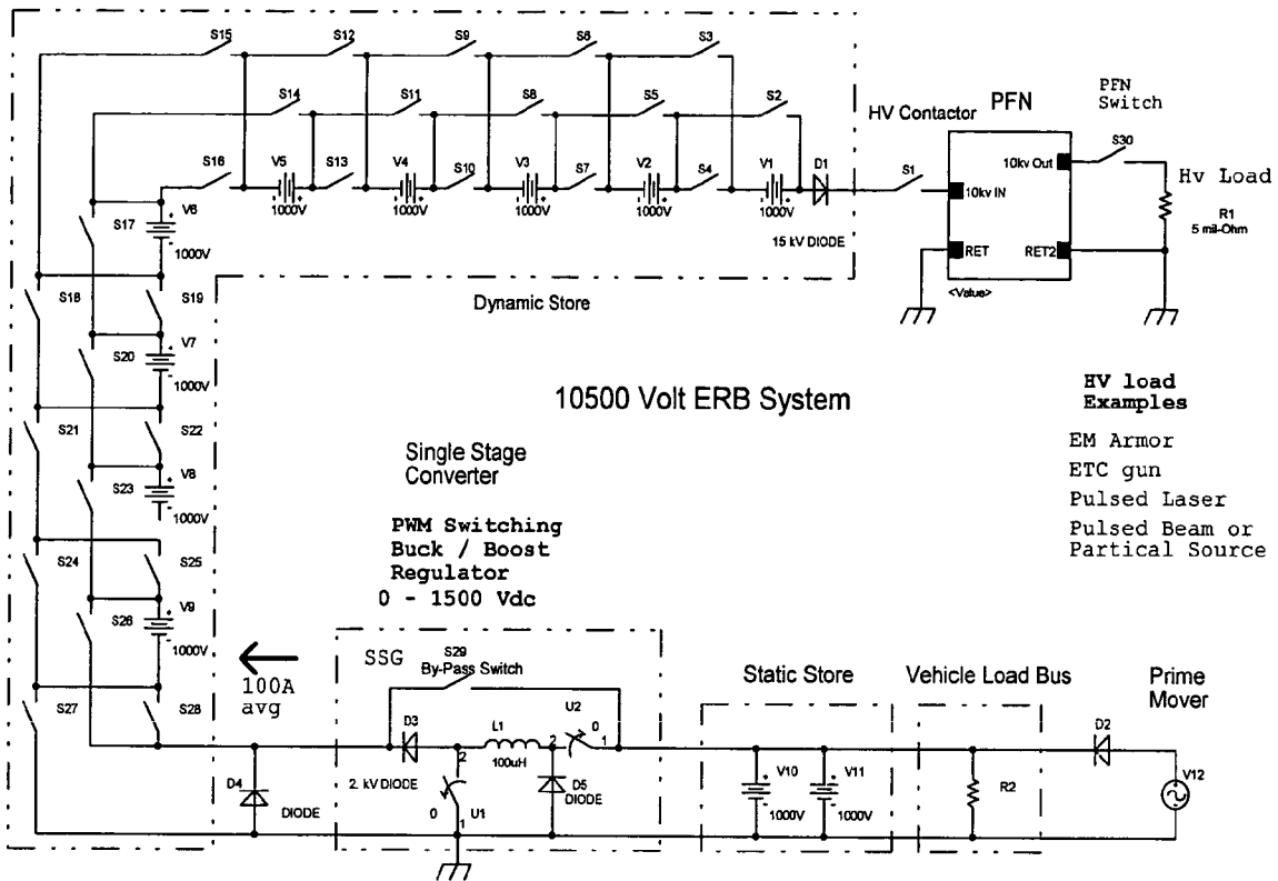
Figure 6 10.5 kV ERB with a single stage Buck\Boost converter.
